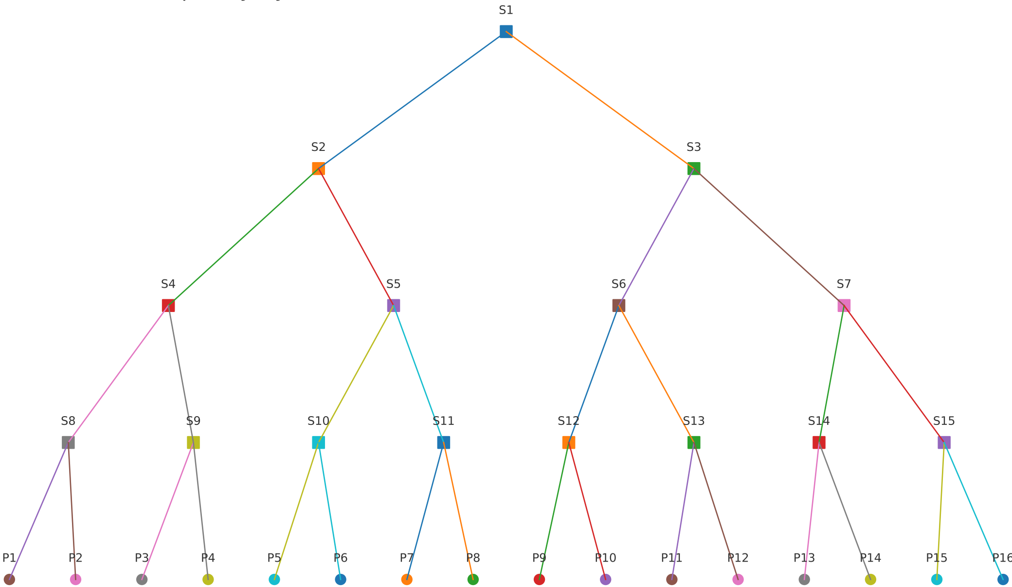
Completely Dynamic Tree Network: 16 Processors (P) + 15 Switches (S)
